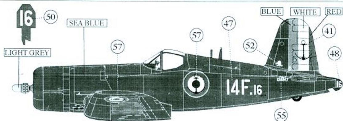
F4U-7, BuNo.133667, Flottile 14, Aeronavale, on board ARROMANCHES 1954
