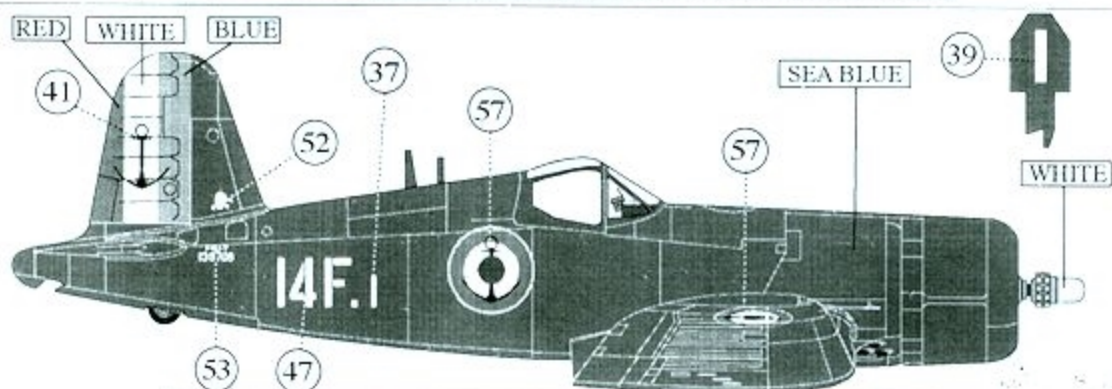
F4U-7, BuNo.133708, Flottile 14, Aeronavale, on board ARROMANCHES 1954
