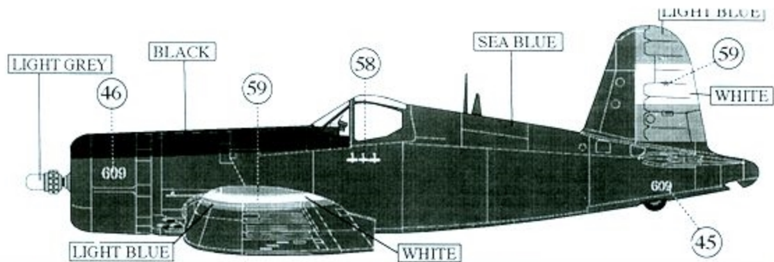
F4U -5, HONDURAN AIR FORCE, Maj. Fernando Soto HENRIQUEZ (3 Kills Salvadorean), "Football War" 1969
