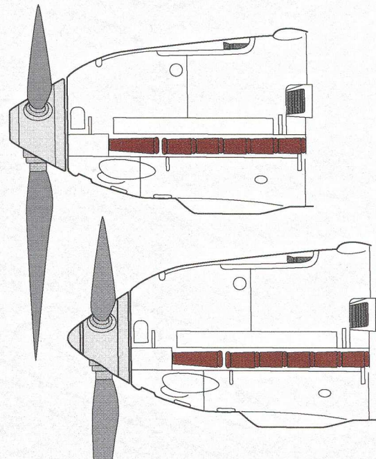
Messerschmitt Bf 109E1 - E7 propeller with tool - TAM / AIRFIX
