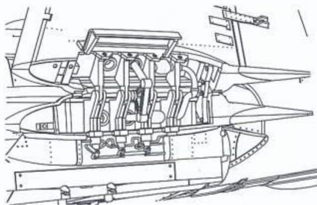
illustration of finished wing fold mechanism
