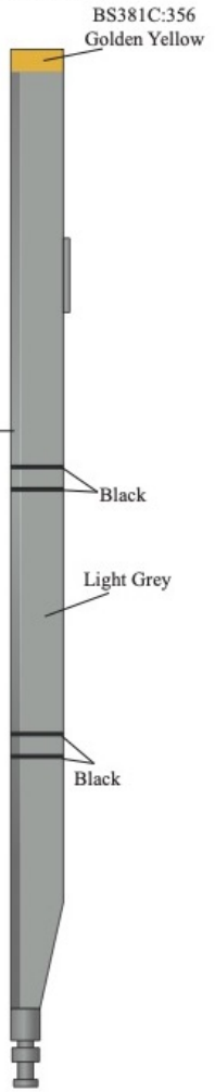
Lowersurfaces of Main Rotor Blades
