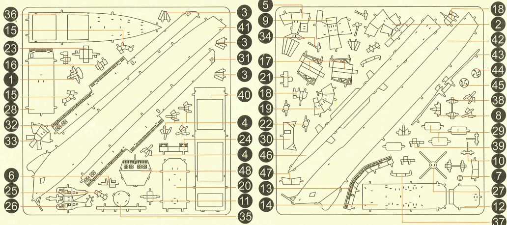
Schematic drawing of sheet metals (two pieces of sheet metals). 金屬片示意圖 (有2片金屬)
