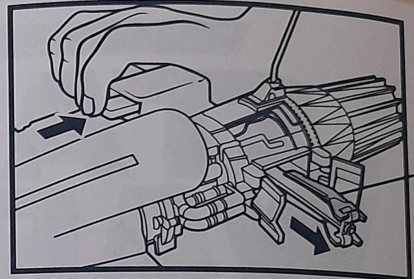
Press button on handle to release blades.
