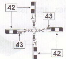
Tail rotor (outboard)
