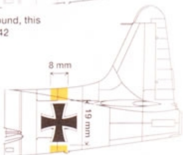
Dimensions for masking Day-Glo band around fuselage insignia.
